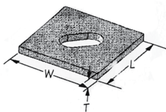
HBPS Slotted Bearing Plate
